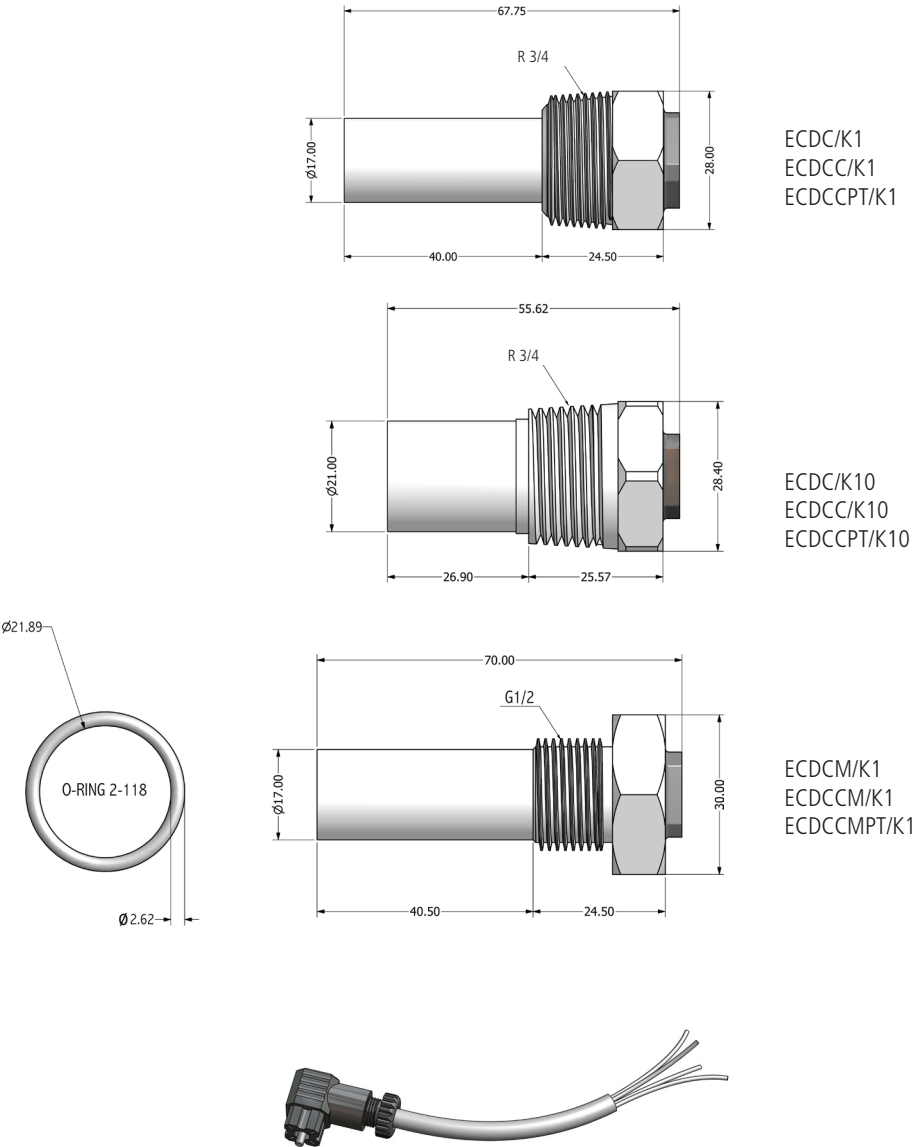
Fig. 6. Dimensions ECDC (mm)
